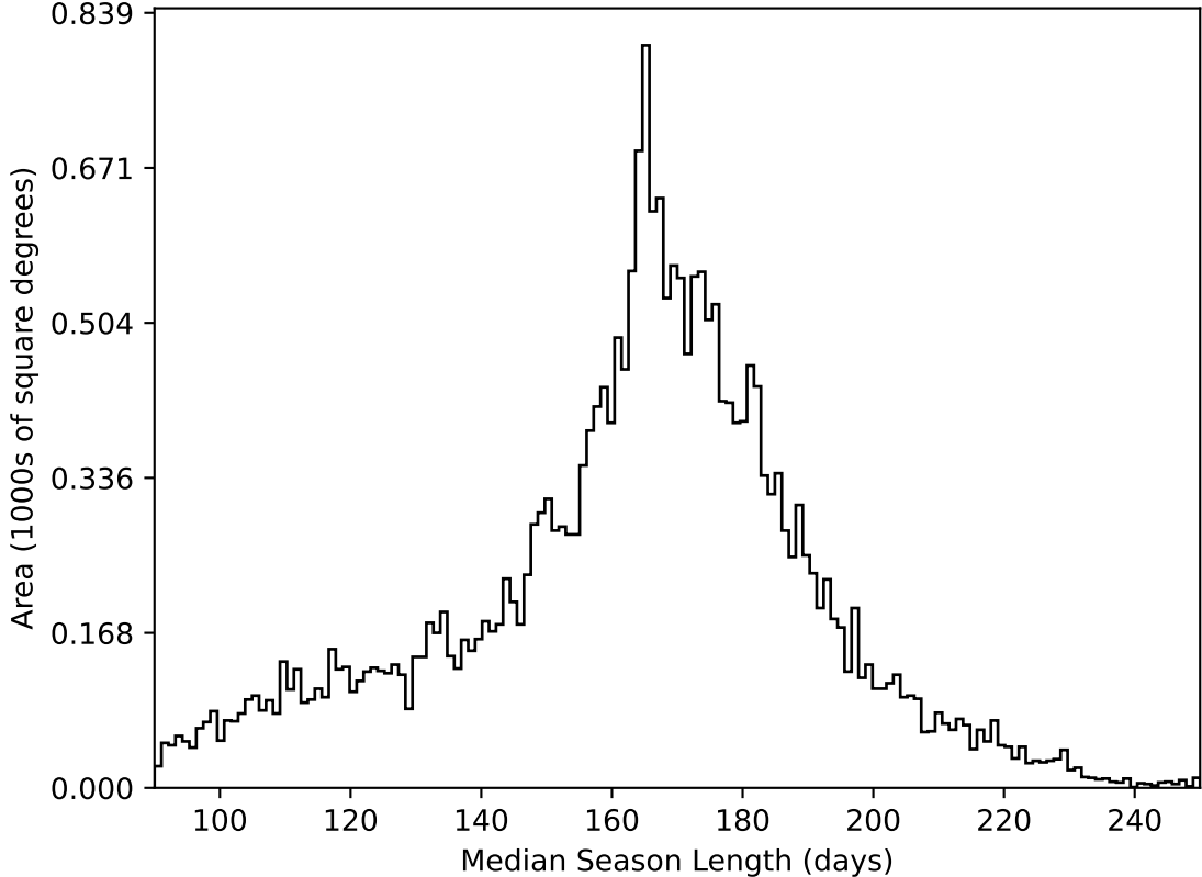
too_elab_heavy_r32_d2_griz_v3.4_10yrs All sky all bands: Median Season Length
