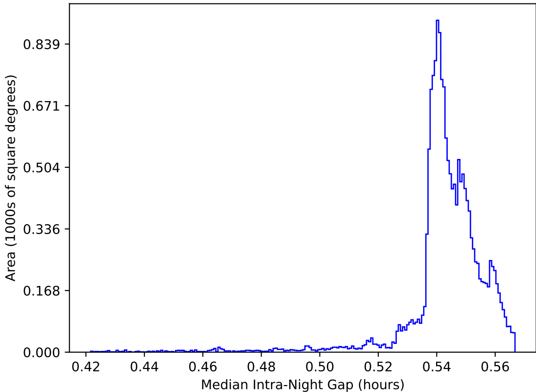
too_elab_heavy_r32_d2_griz_v3.4_10yrs WFD: Median Intra-Night Gap
