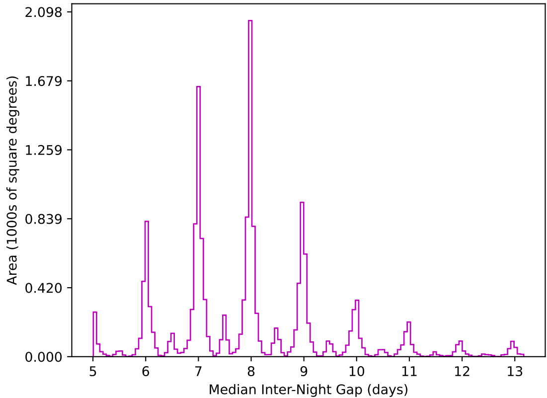
too_elab_heavy_r32_d2_griz_v3.4_10yrs WFD z band: Median Inter-Night Gap
