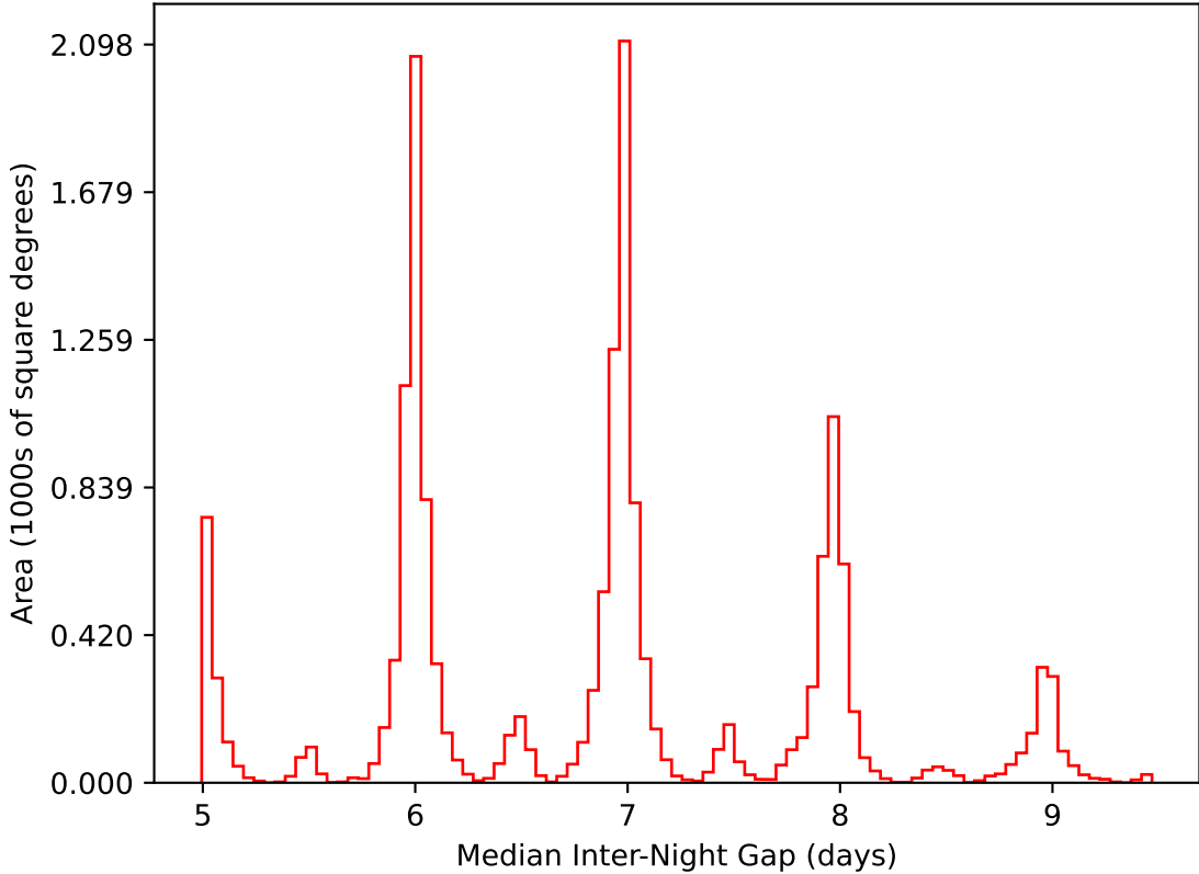
too_elab_heavy_r32_d2_griz_v3.4_10yrs WFD i band: Median Inter-Night Gap
