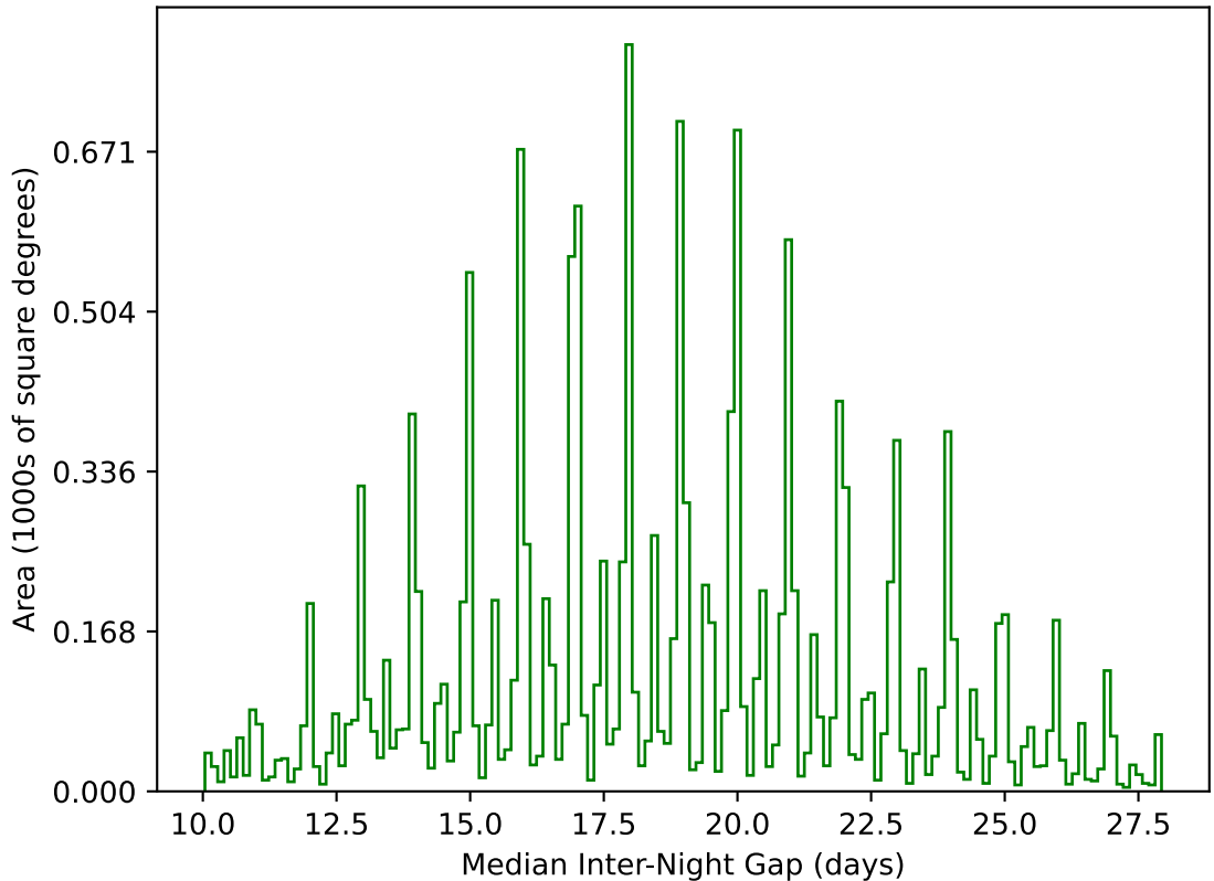
too_elab_heavy_r32_d2_griz_v3.4_10yrs WFD g band: Median Inter-Night Gap
