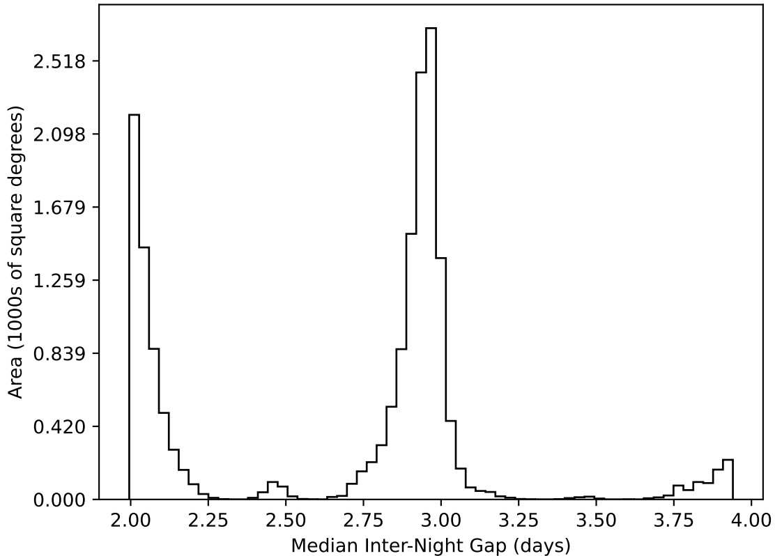
too_elab_heavy_r32_d2_griz_v3.4_10yrs WFD all bands: Median Inter-Night Gap
