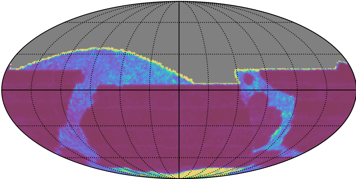
too_elab_heavy_r32_d2_griz_v3.4_10yrs All sky i band: Median Inter-Night Gap
