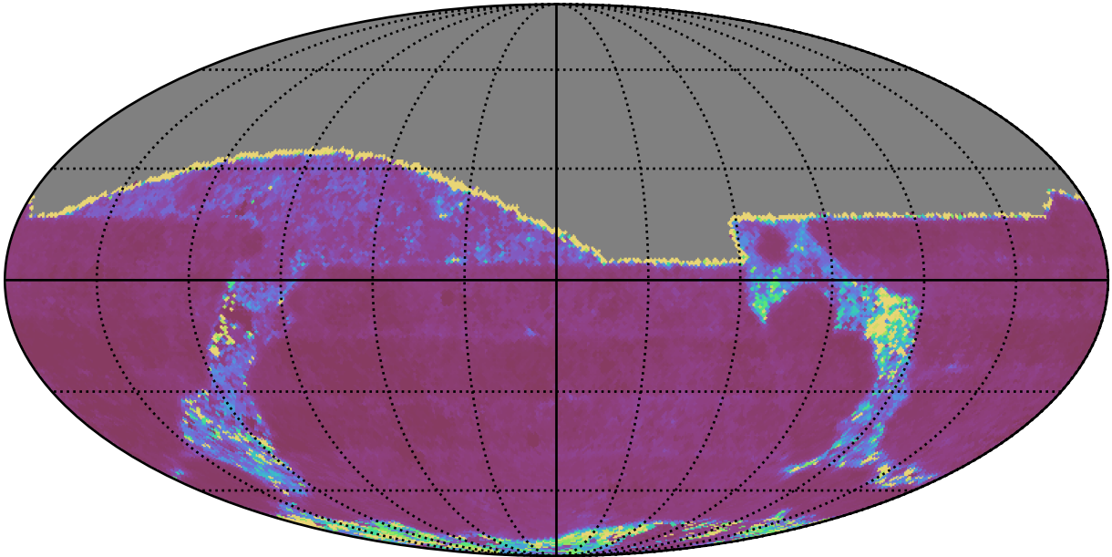
too_elab_heavy_r32_d2_griz_v3.4_10yrs All sky g band: Median Inter-Night Gap
