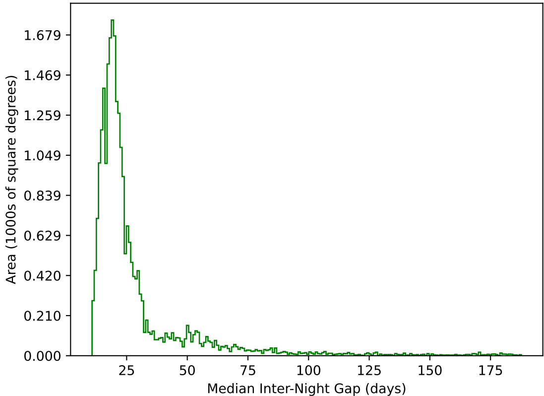
too_elab_heavy_r32_d2_griz_v3.4_10yrs All sky g band: Median Inter-Night Gap
