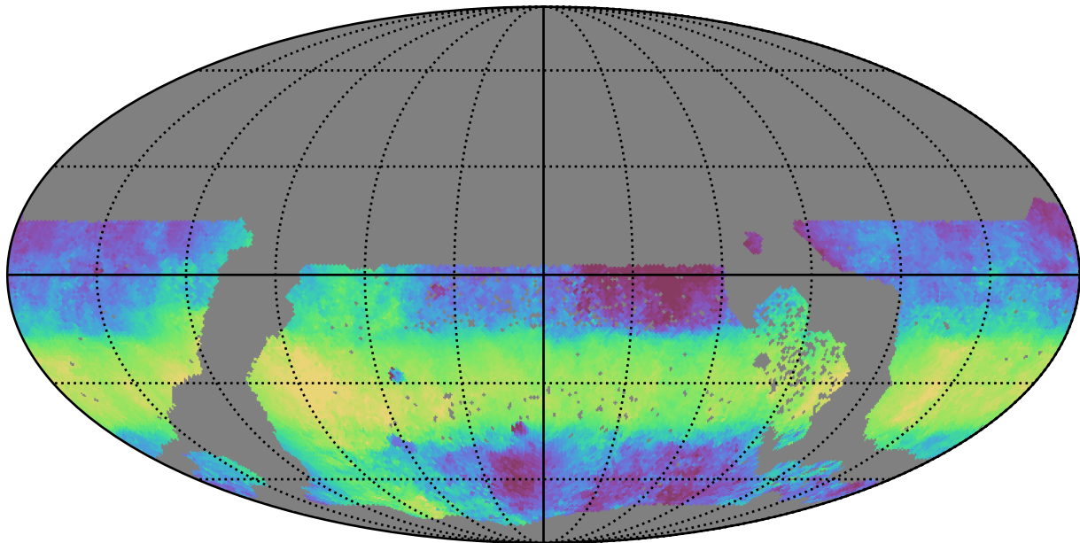
too_elab_heavy_r32_d2_griz_v3.4_10yrs WFD y band: Median HA
