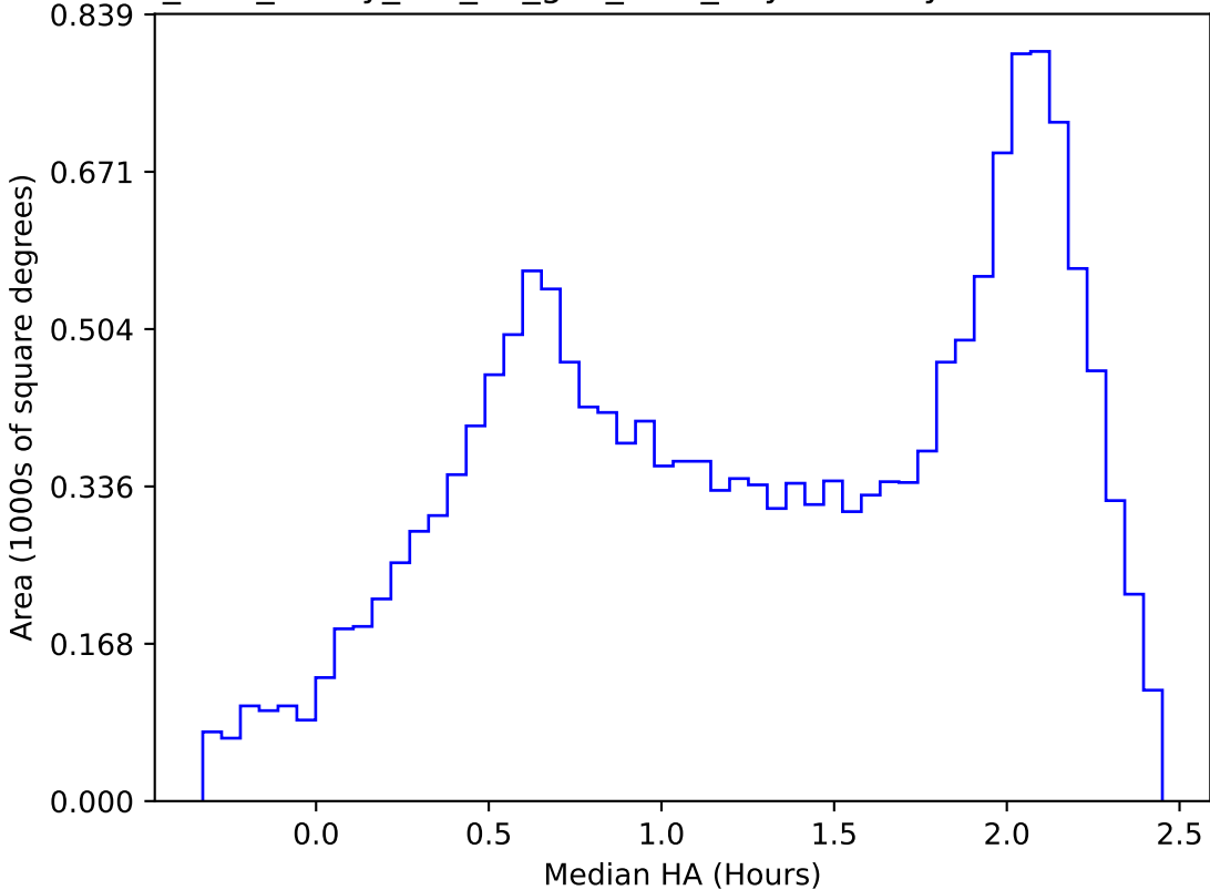
too_elab_heavy_r32_d2_griz_v3.4_10yrs WFD y band: Median HA
