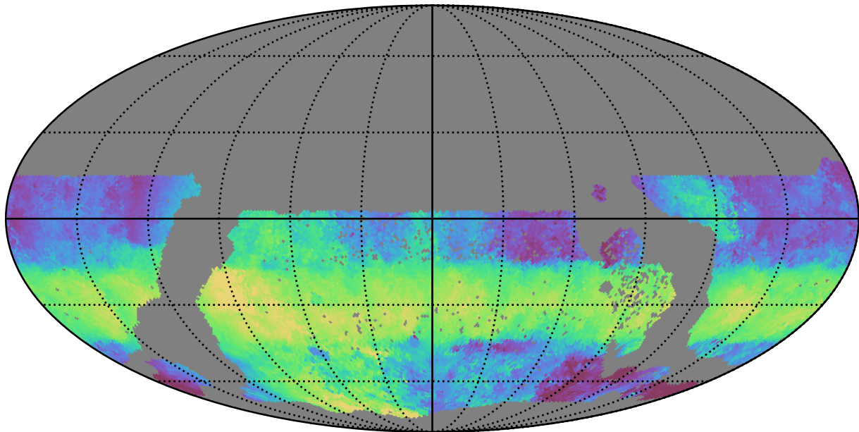
too_elab_heavy_r32_d2_griz_v3.4_10yrs WFD u band: Median HA
