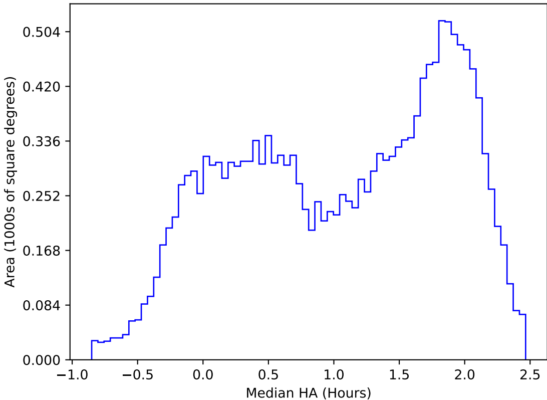
too_elab_heavy_r32_d2_griz_v3.4_10yrs WFD u band: Median HA
