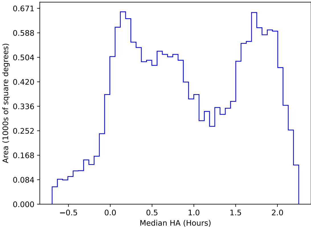
too_elab_heavy_r32_d2_griz_v3.4_10yrs WFD r band: Median HA
