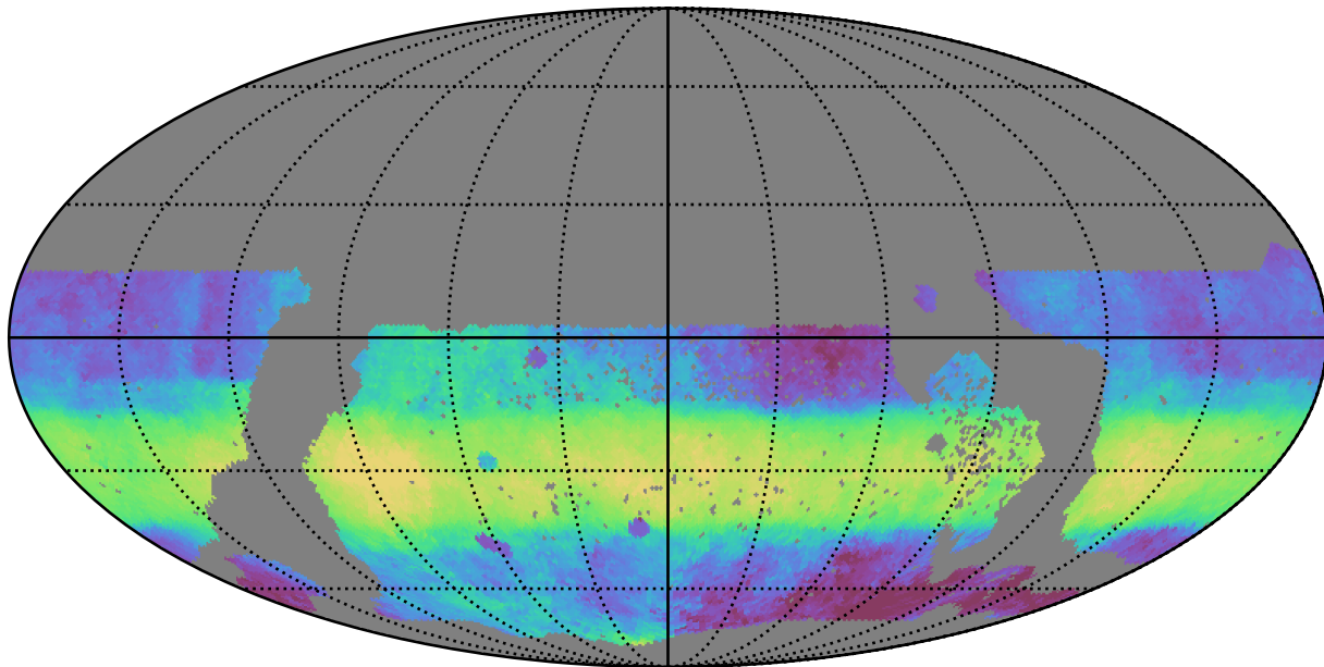
too_elab_heavy_r32_d2_griz_v3.4_10yrs WFD i band: Median HA
