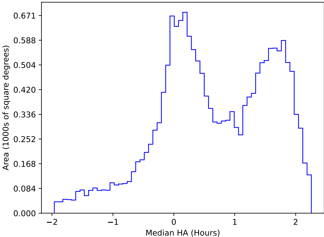
too_elab_heavy_r32_d2_griz_v3.4_10yrs WFD g band: Median HA
