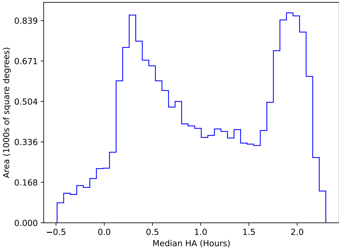
too_elab_heavy_r32_d2_griz_v3.4_10yrs WFD all bands: Median HA
