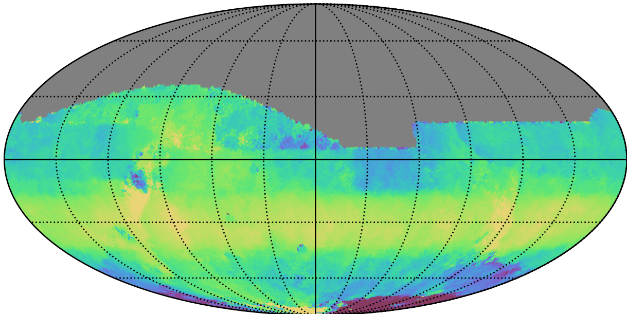
too_elab_heavy_r32_d2_griz_v3.4_10yrs All sky z band: Median HA
