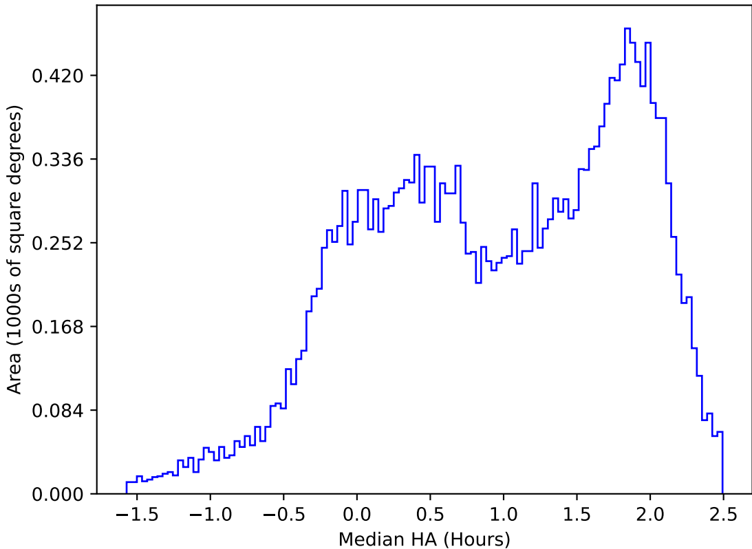
too_elab_heavy_r32_d2_griz_v3.4_10yrs All sky u band: Median HA
