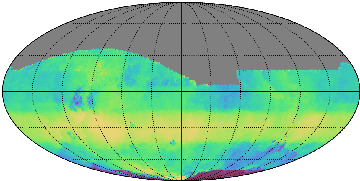
too_elab_heavy_r32_d2_griz_v3.4_10yrs All sky r band: Median HA
