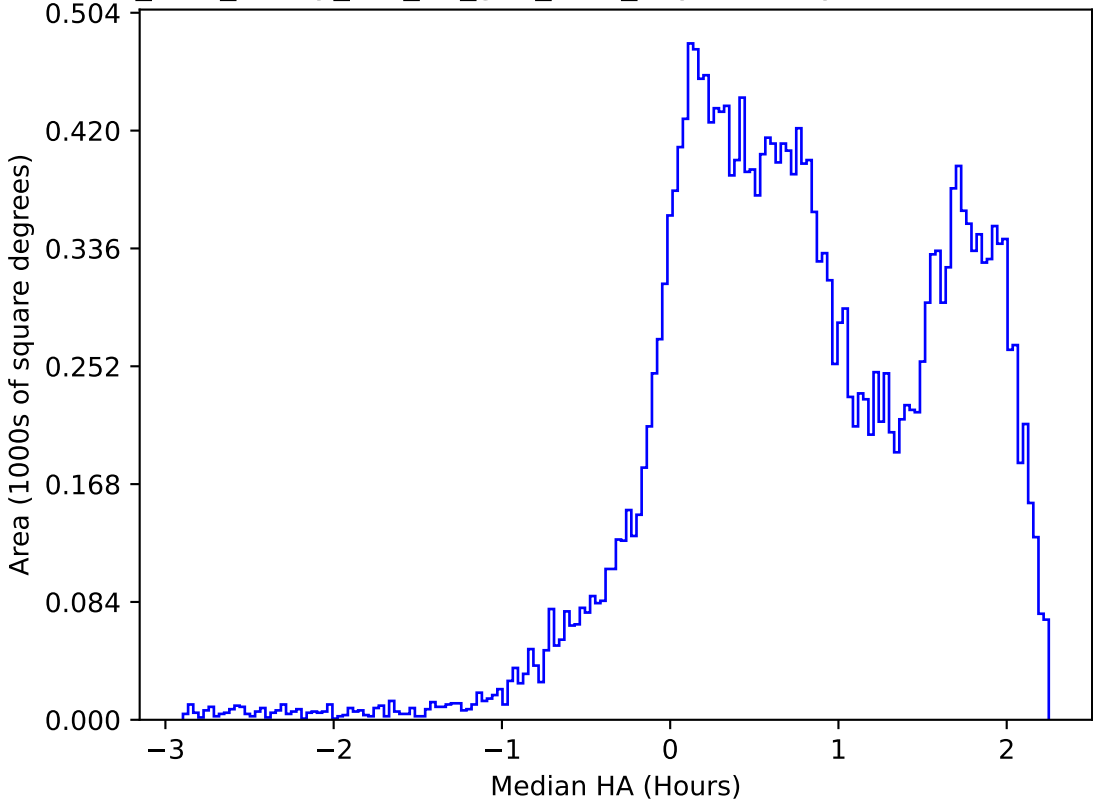
too_elab_heavy_r32_d2_griz_v3.4_10yrs All sky r band: Median HA
