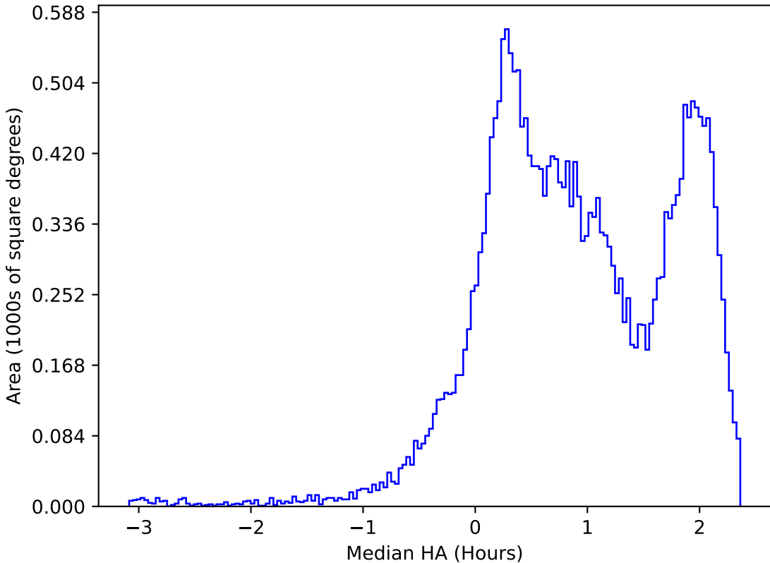
too_elab_heavy_r32_d2_griz_v3.4_10yrs All sky i band: Median HA
