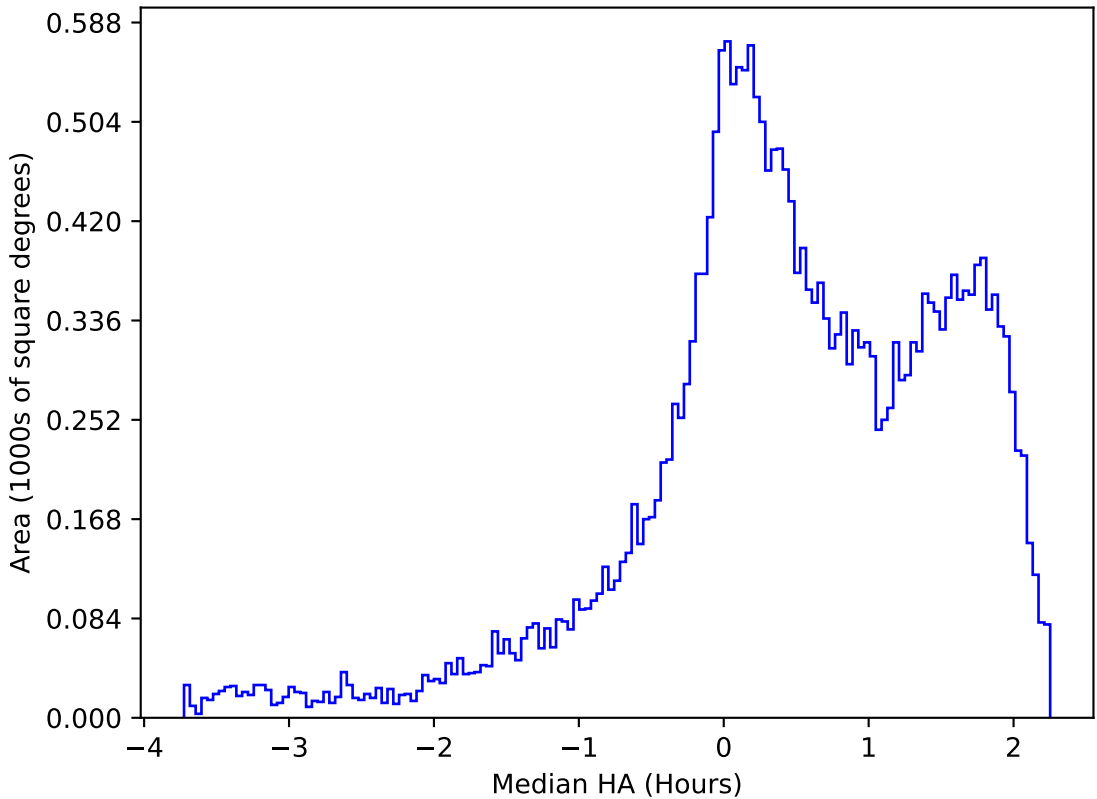
too_elab_heavy_r32_d2_griz_v3.4_10yrs All sky g band: Median HA
