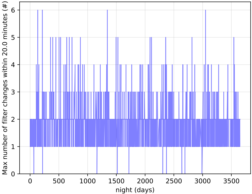
too_elab_heavy_r32_d2_griz_v3.4_10yrs Per Night: Max number of filter changes within 20.0 minutes
