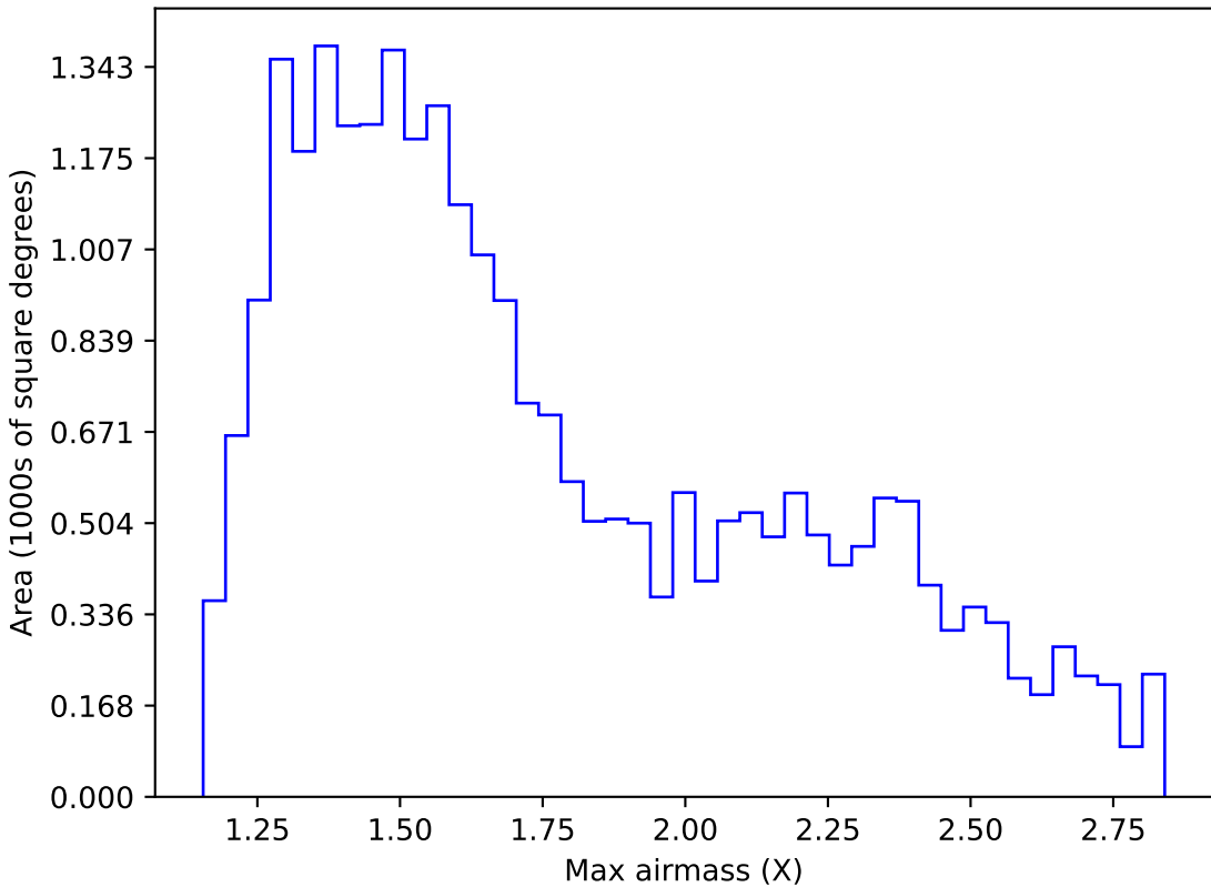
too_elab_heavy_r32_d2_griz_v3.4_10yrs Yr 1 z band: Max airmass
