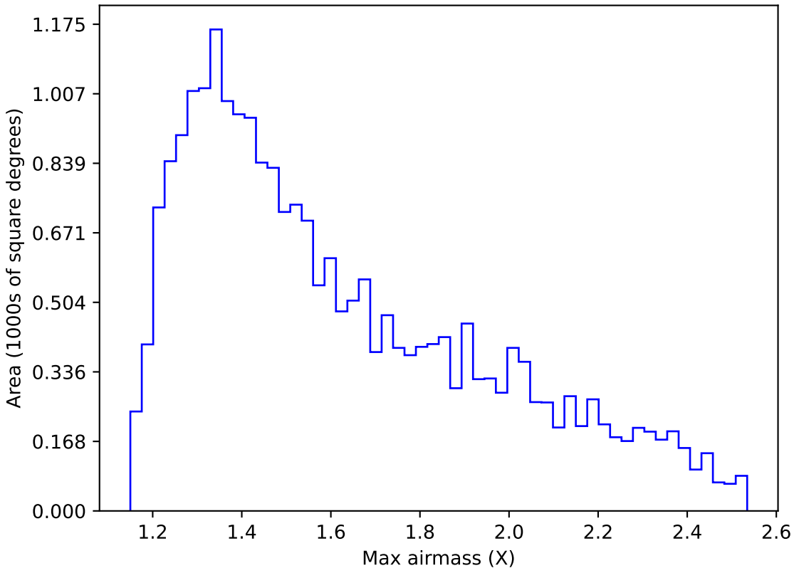
too_elab_heavy_r32_d2_griz_v3.4_10yrs Yr 1 y band: Max airmass
