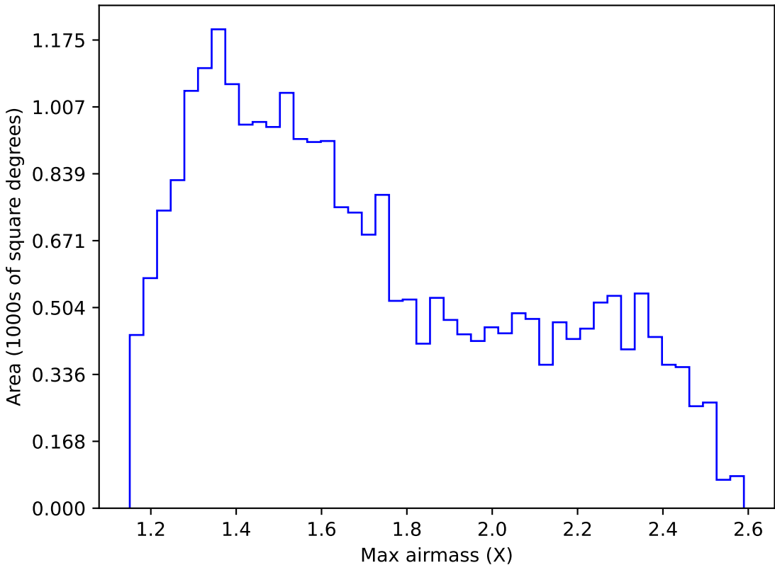
too_elab_heavy_r32_d2_griz_v3.4_10yrs Yr 1 r band: Max airmass
