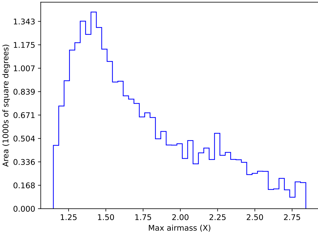
too_elab_heavy_r32_d2_griz_v3.4_10yrs Yr 1 i band: Max airmass
