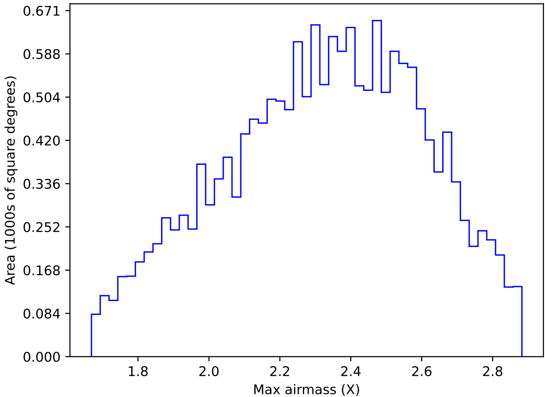
too_elab_heavy_r32_d2_griz_v3.4_10yrs WFD y band: Max airmass
