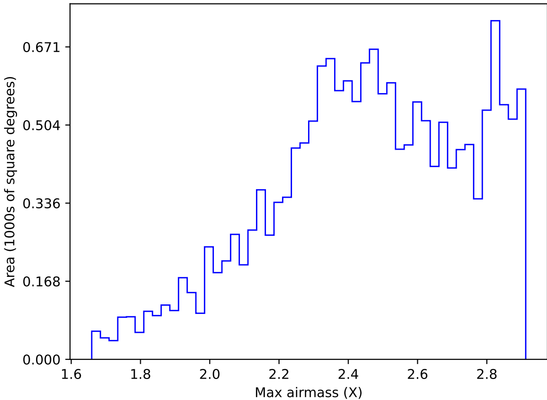
too_elab_heavy_r32_d2_griz_v3.4_10yrs WFD i band: Max airmass
