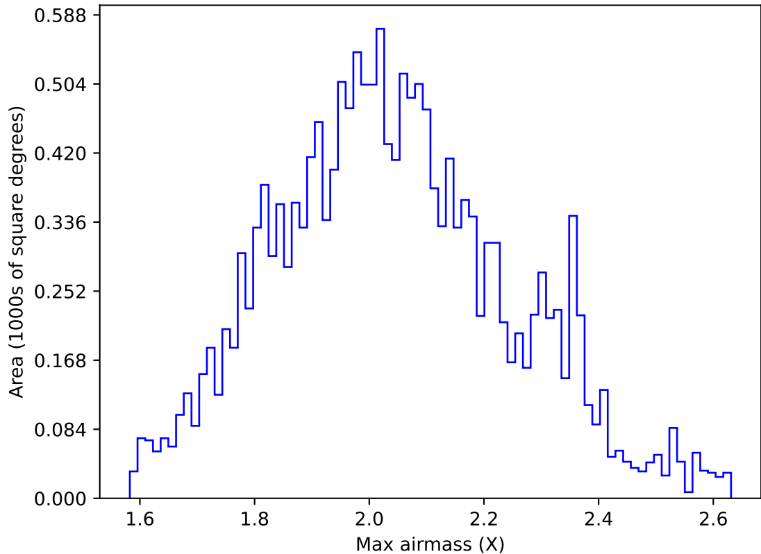
too_elab_heavy_r32_d2_griz_v3.4_10yrs WFD g band: Max airmass
