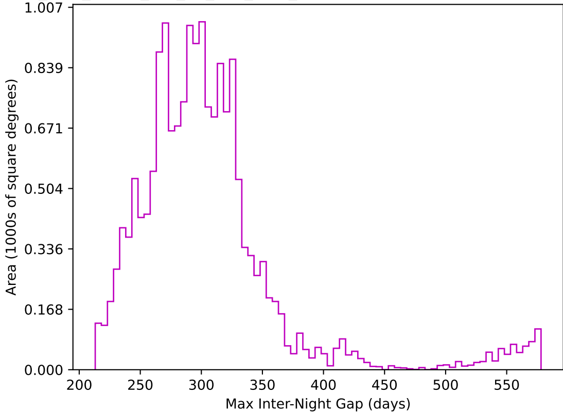
too_elab_heavy_r32_d2_griz_v3.4_10yrs WFD z band: Max Inter-Night Gap
