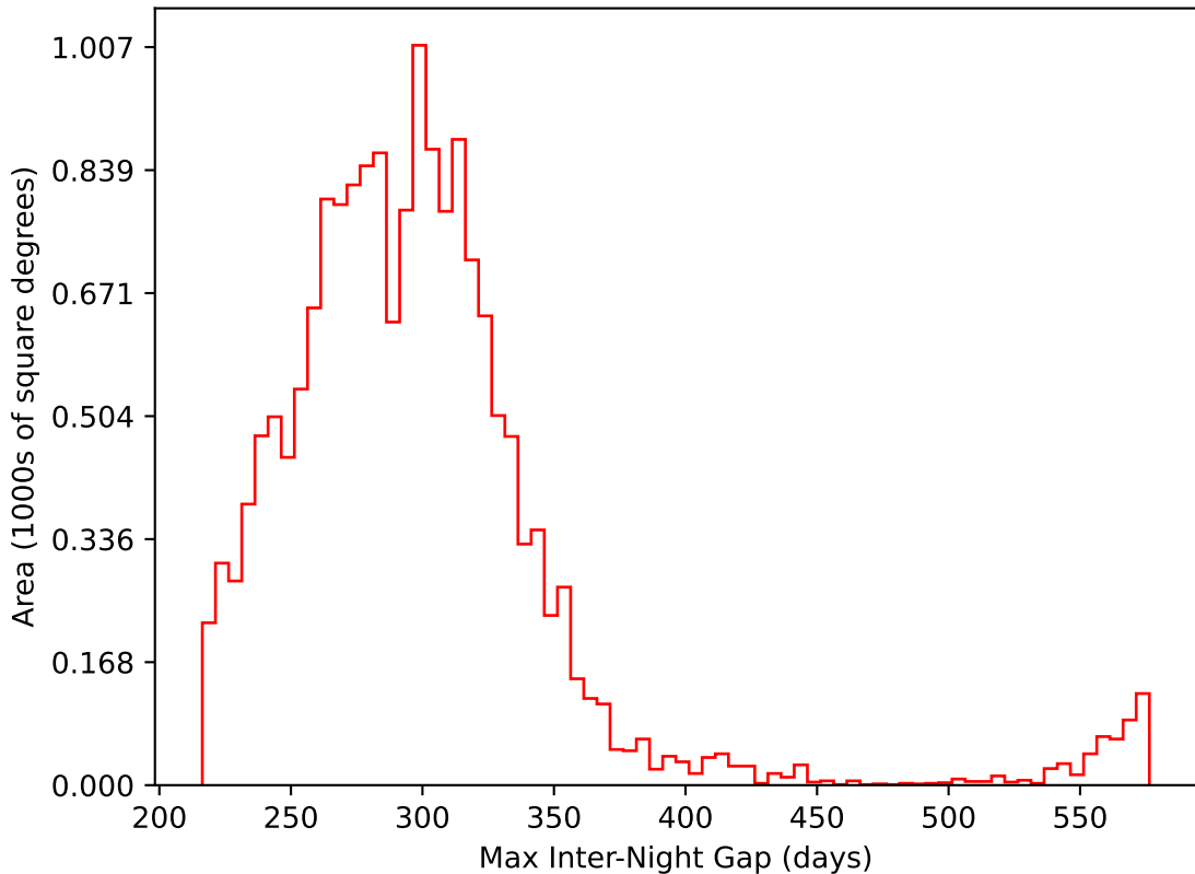
too_elab_heavy_r32_d2_griz_v3.4_10yrs WFD i band: Max Inter-Night Gap
