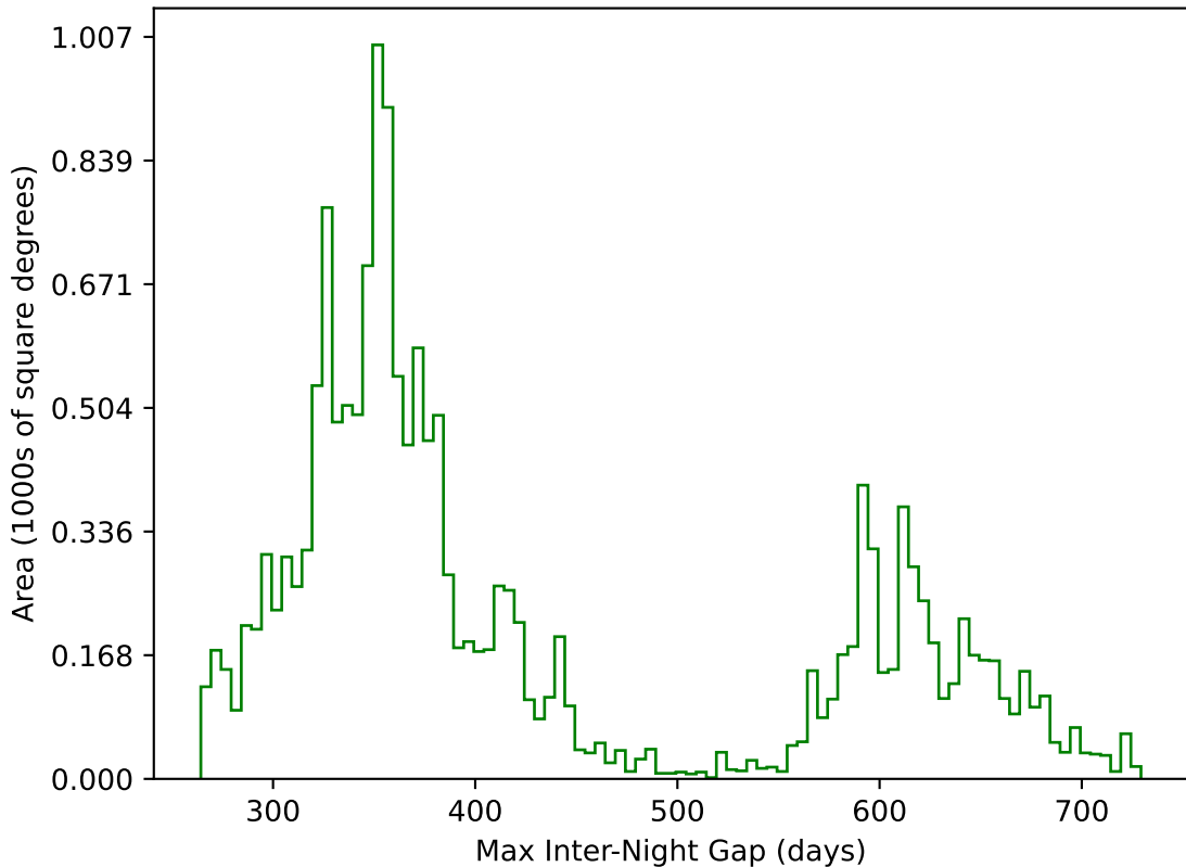
too_elab_heavy_r32_d2_griz_v3.4_10yrs WFD g band: Max Inter-Night Gap
