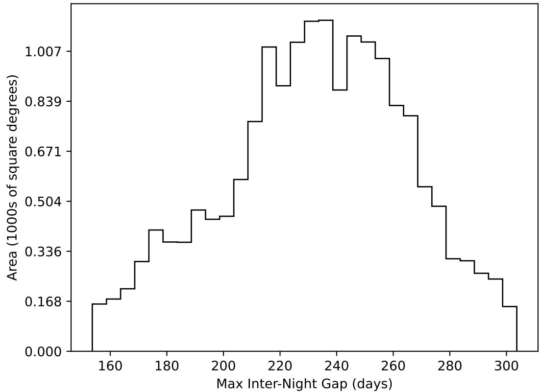
too_elab_heavy_r32_d2_griz_v3.4_10yrs WFD all bands: Max Inter-Night Gap
