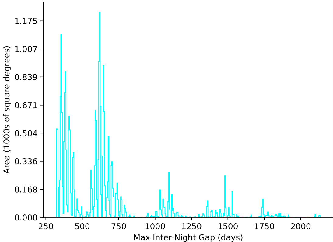
too_elab_heavy_r32_d2_griz_v3.4_10yrs All sky u band: Max Inter-Night Gap
