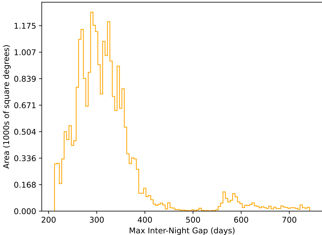
too_elab_heavy_r32_d2_griz_v3.4_10yrs All sky r band: Max Inter-Night Gap
