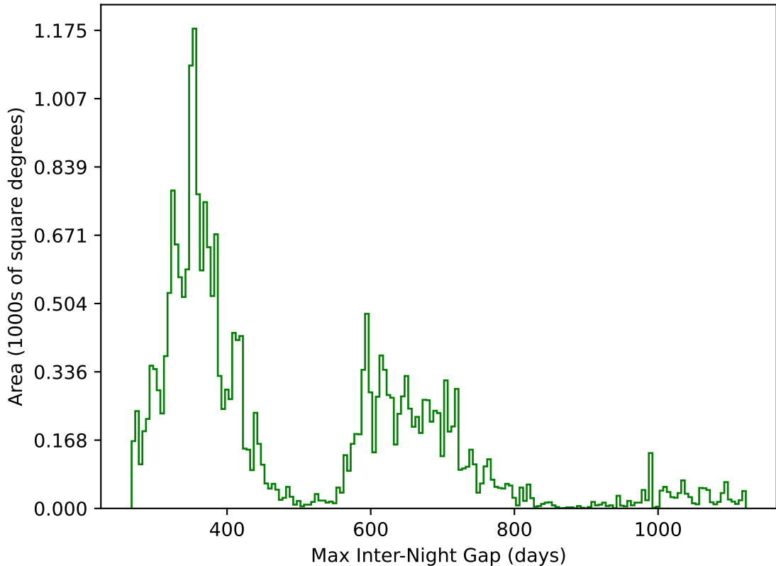
too_elab_heavy_r32_d2_griz_v3.4_10yrs All sky g band: Max Inter-Night Gap
