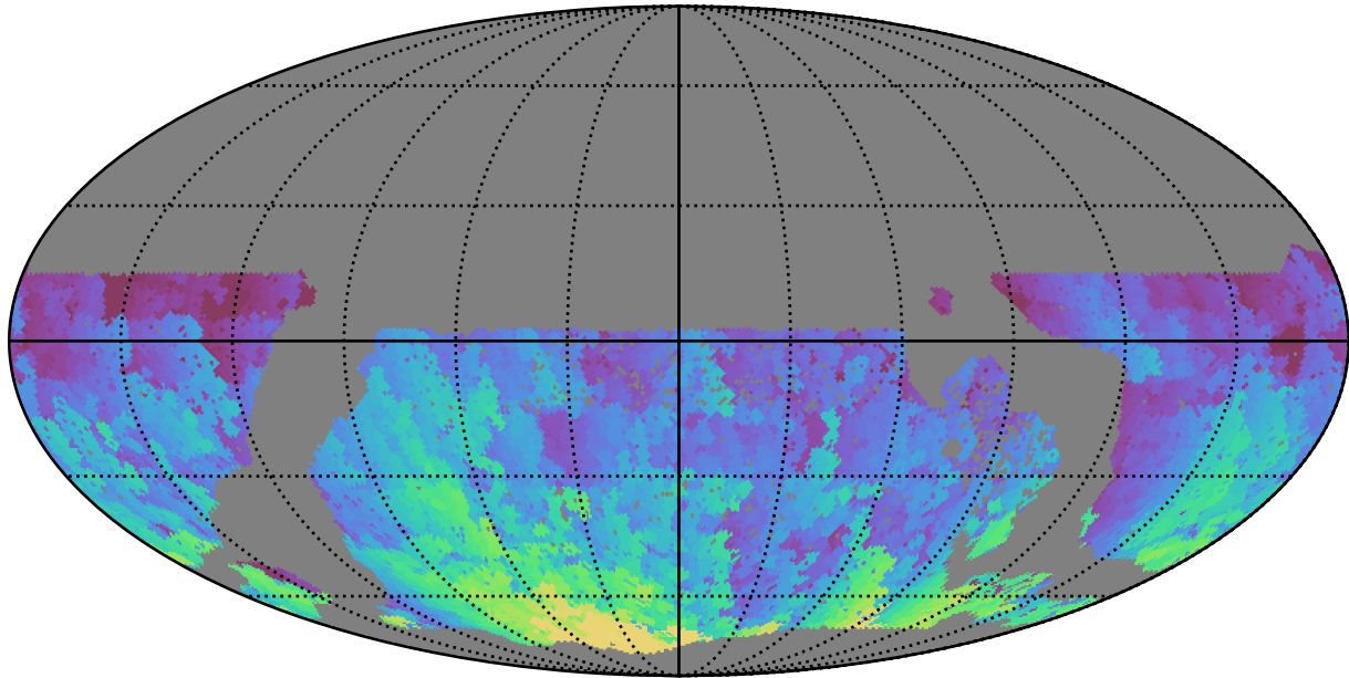
too_elab_heavy_r32_d2_griz_v3.4_10yrs WFD u band: Max HA
