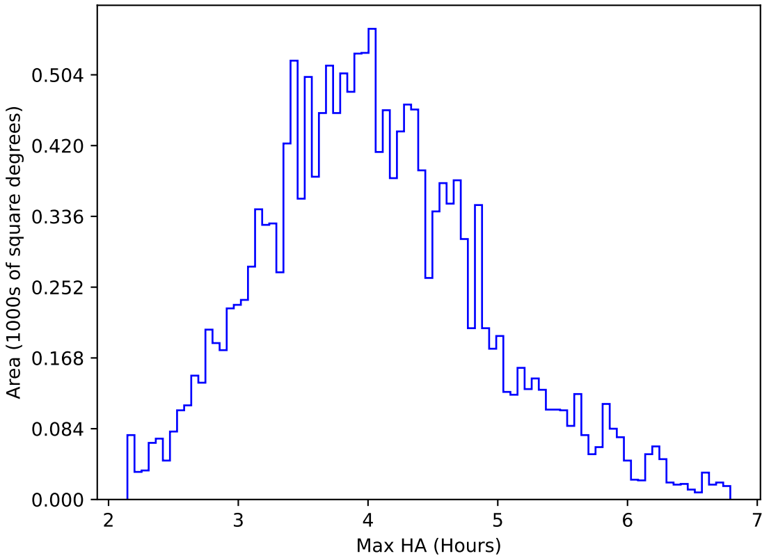
too_elab_heavy_r32_d2_griz_v3.4_10yrs WFD u band: Max HA
