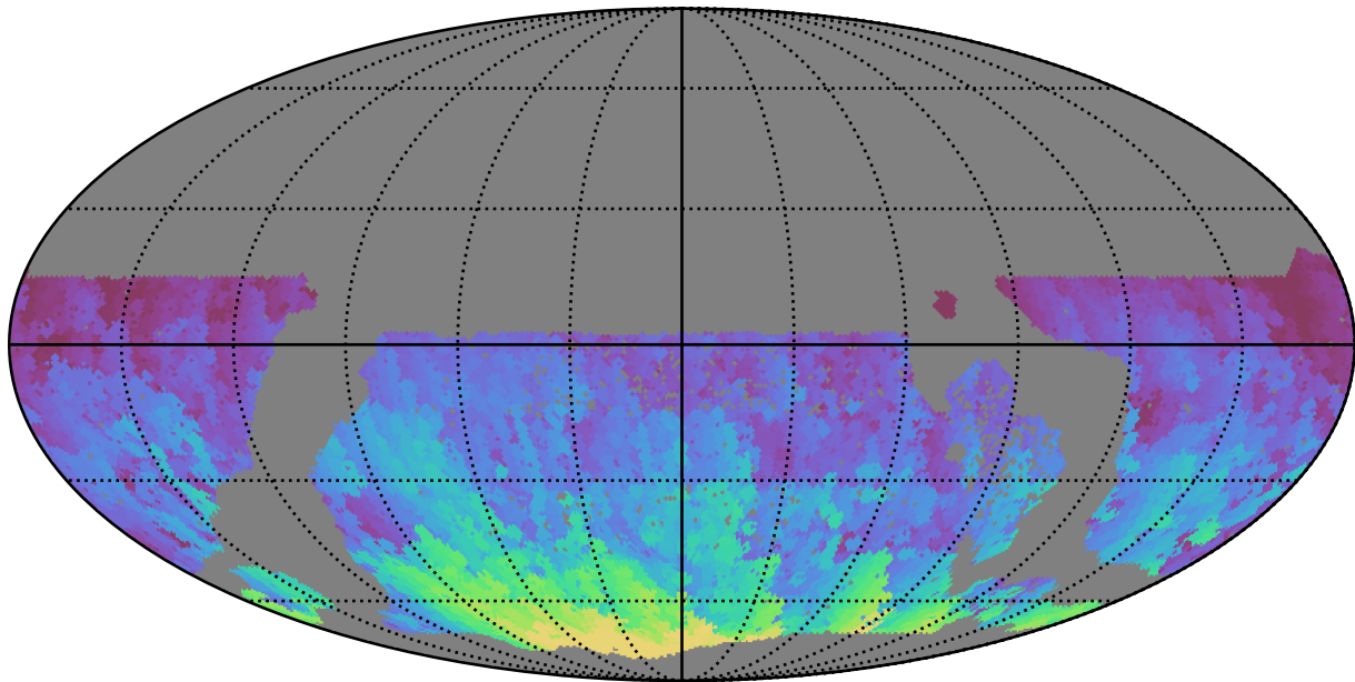
too_elab_heavy_r32_d2_griz_v3.4_10yrs WFD r band: Max HA
