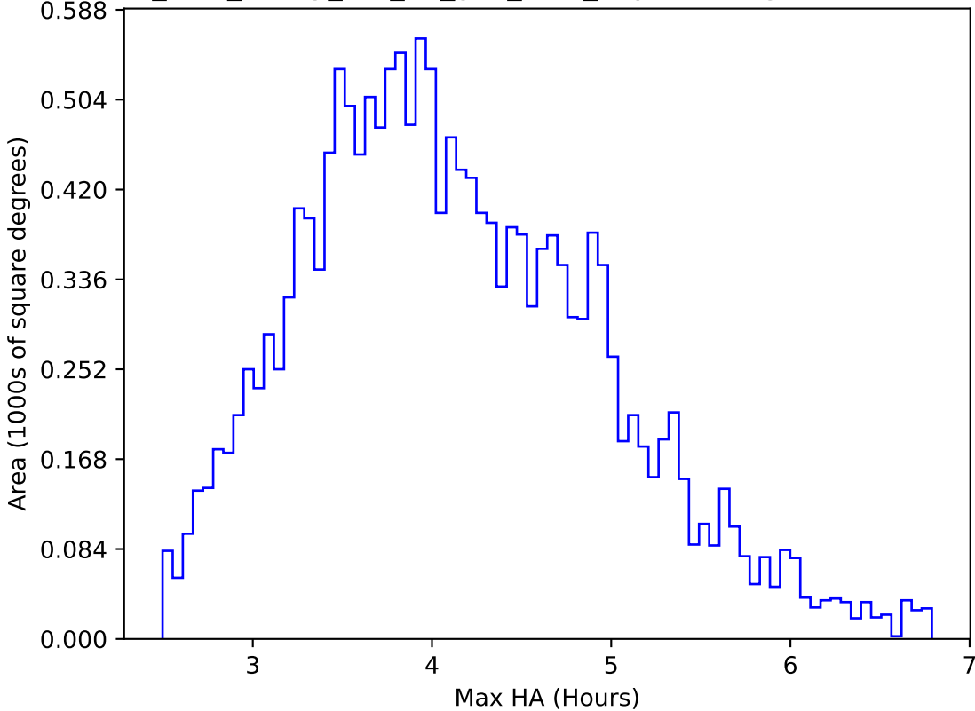
too_elab_heavy_r32_d2_griz_v3.4_10yrs WFD g band: Max HA
