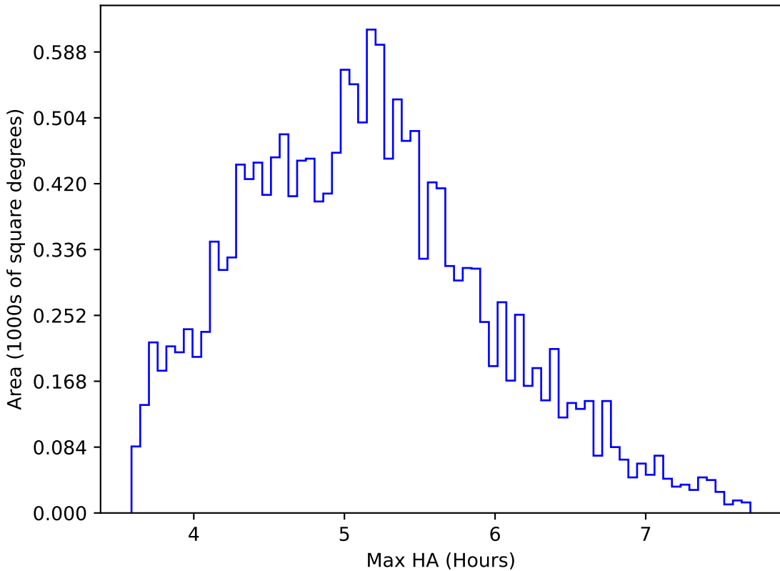
too_elab_heavy_r32_d2_griz_v3.4_10yrs WFD all bands: Max HA
