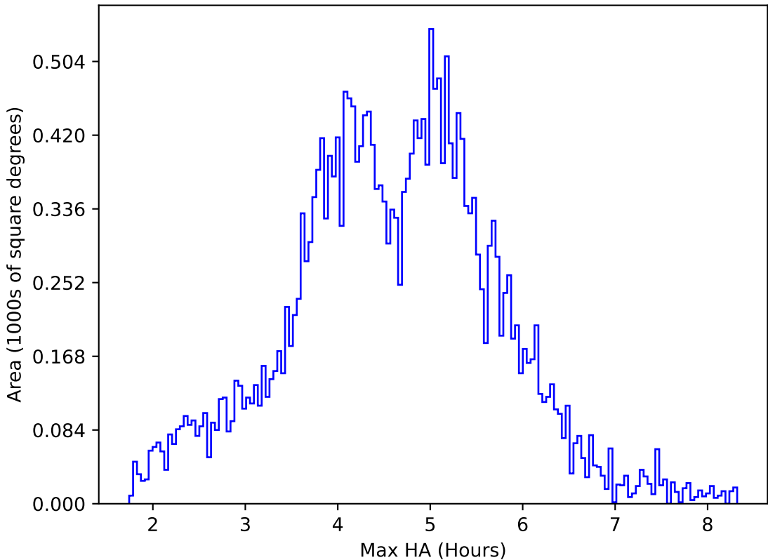
too_elab_heavy_r32_d2_griz_v3.4_10yrs All sky z band: Max HA
