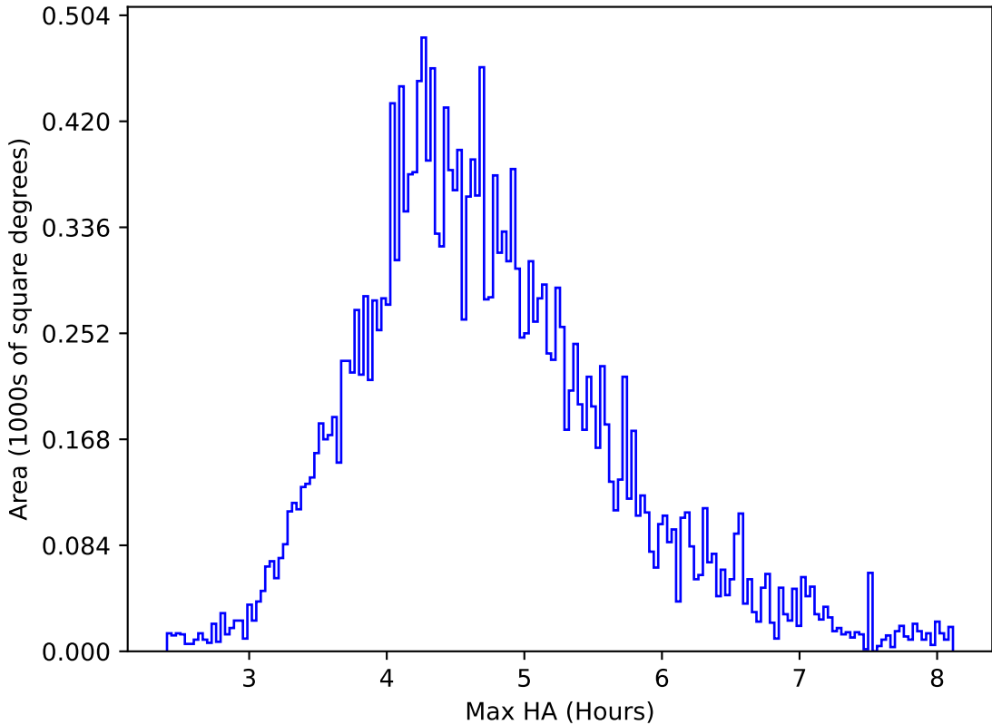
too_elab_heavy_r32_d2_griz_v3.4_10yrs All sky y band: Max HA
