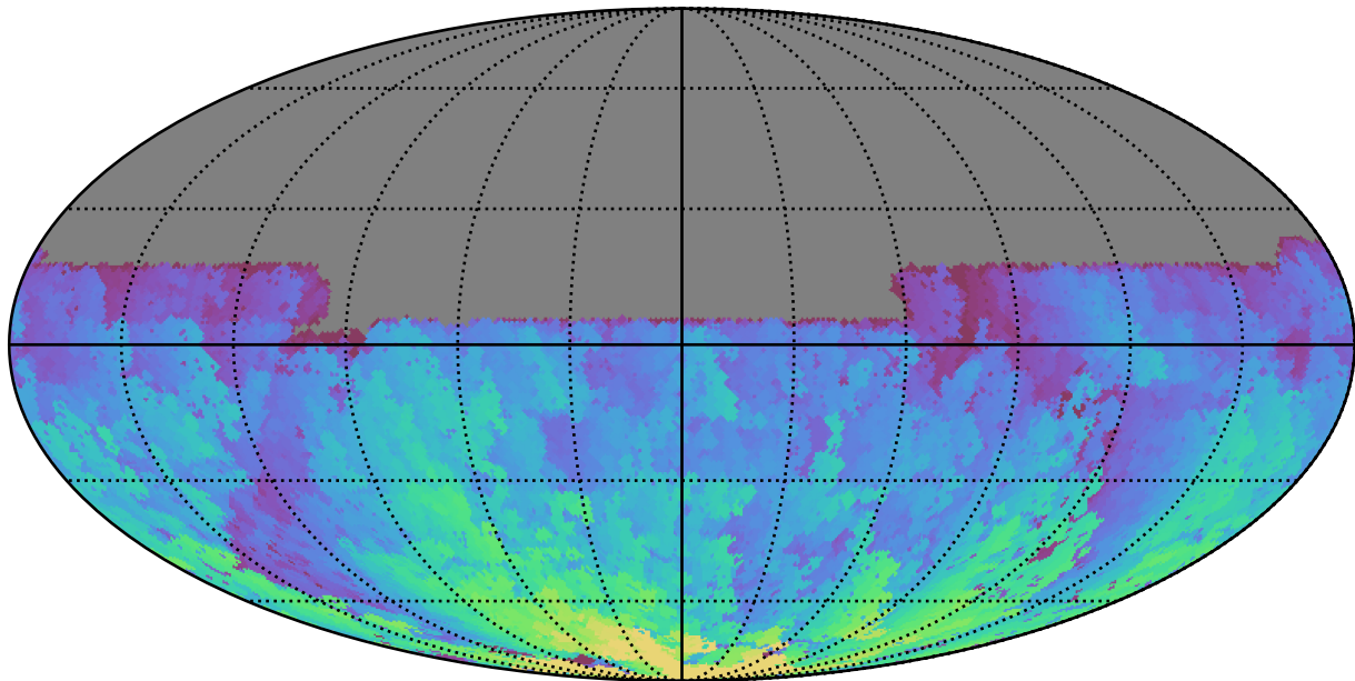
too_elab_heavy_r32_d2_griz_v3.4_10yrs All sky u band: Max HA
