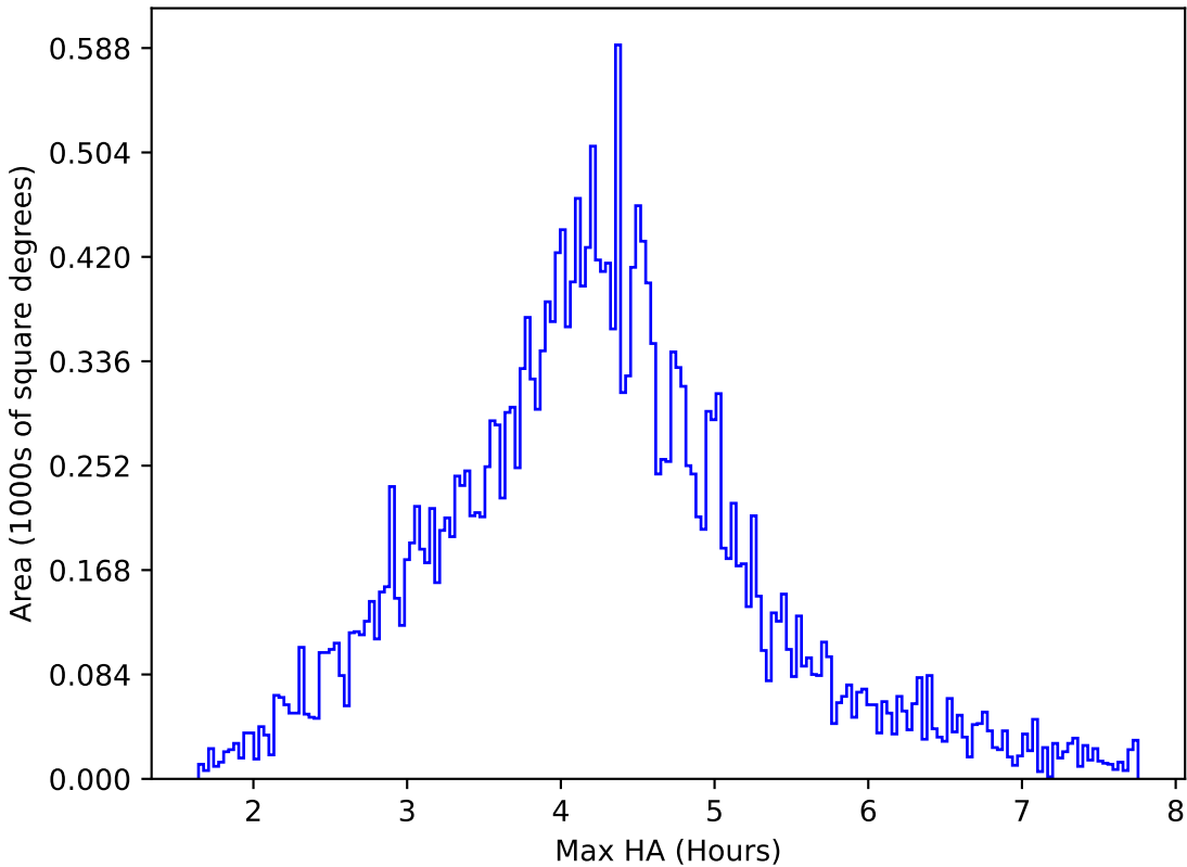
too_elab_heavy_r32_d2_griz_v3.4_10yrs All sky r band: Max HA
