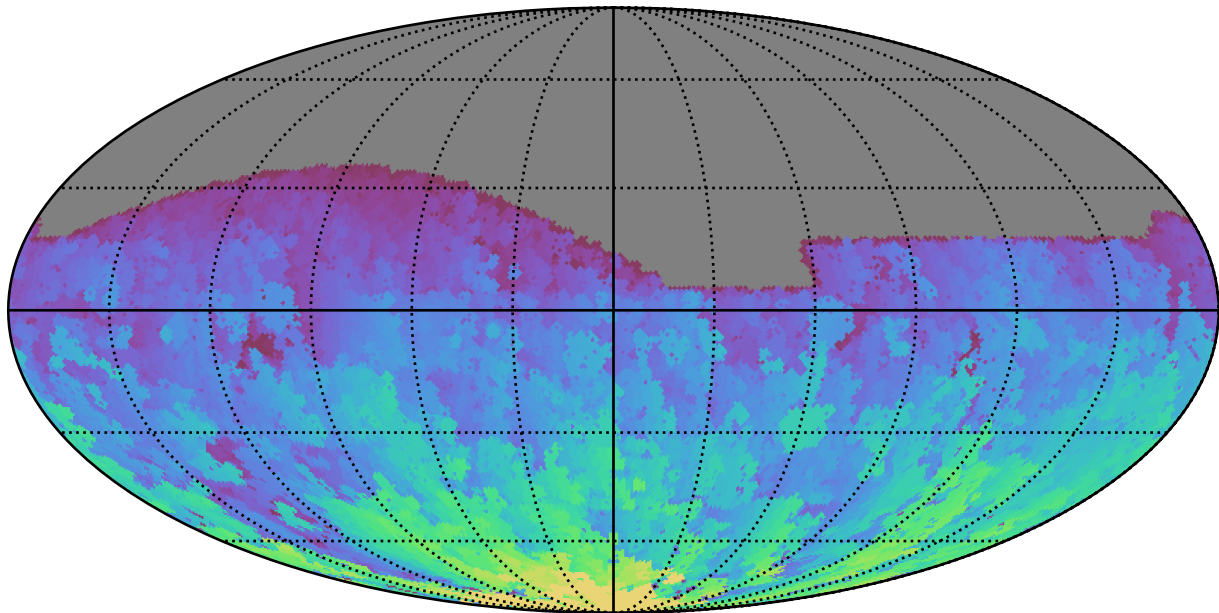
too_elab_heavy_r32_d2_griz_v3.4_10yrs All sky g band: Max HA
