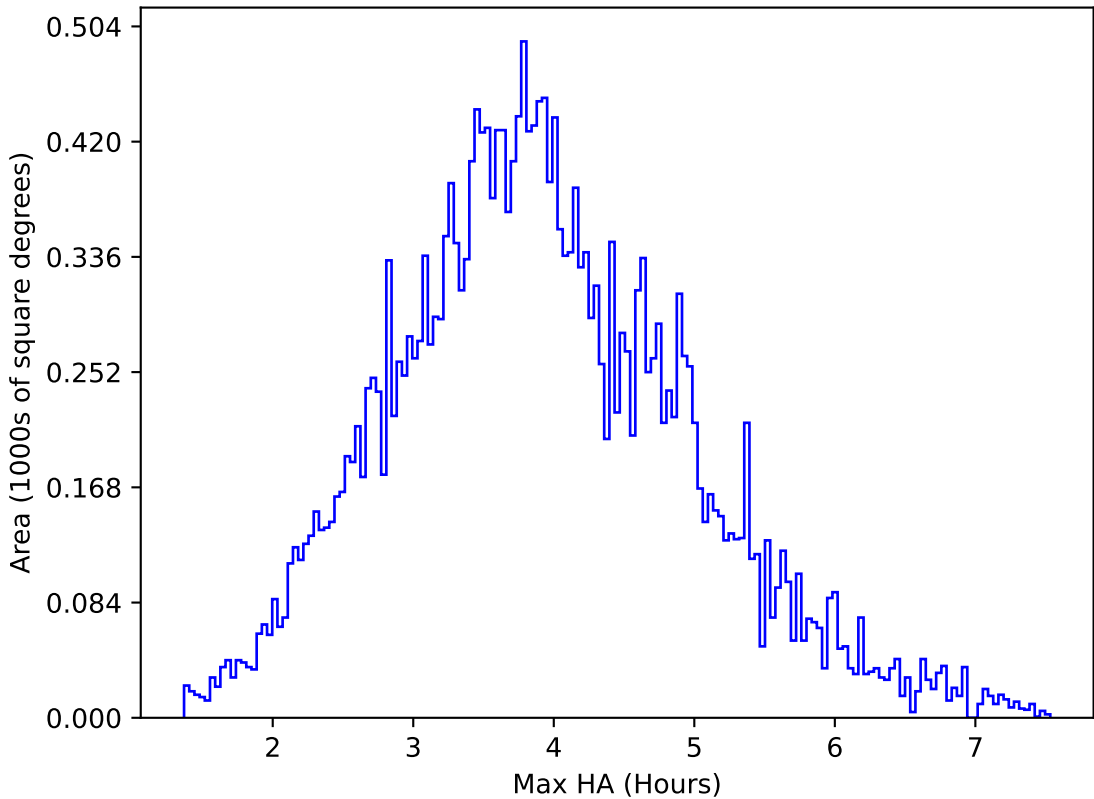
too_elab_heavy_r32_d2_griz_v3.4_10yrs All sky g band: Max HA
