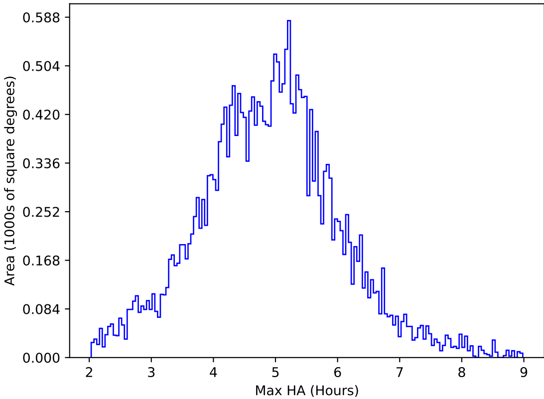
too_elab_heavy_r32_d2_griz_v3.4_10yrs All sky all bands: Max HA
